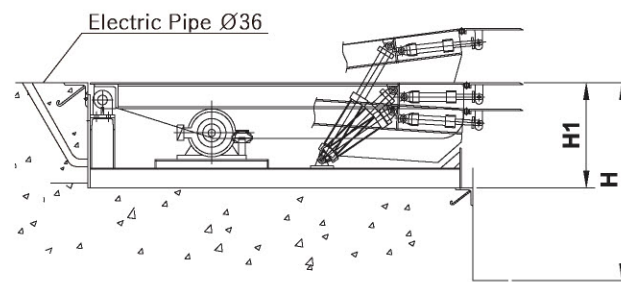
단면도 (Sectional Drawing)
