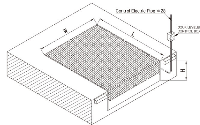
입면도 (Elevation Drawing)
